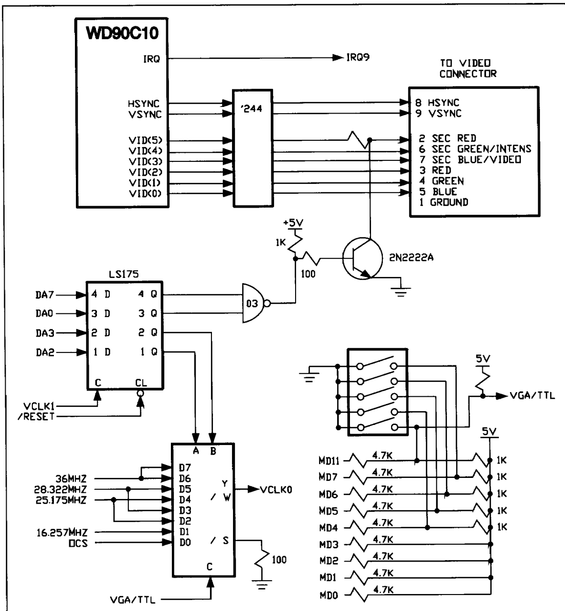
FIGURE 16. WD90C10 AND TTL MONITOR CONNECTIONS
