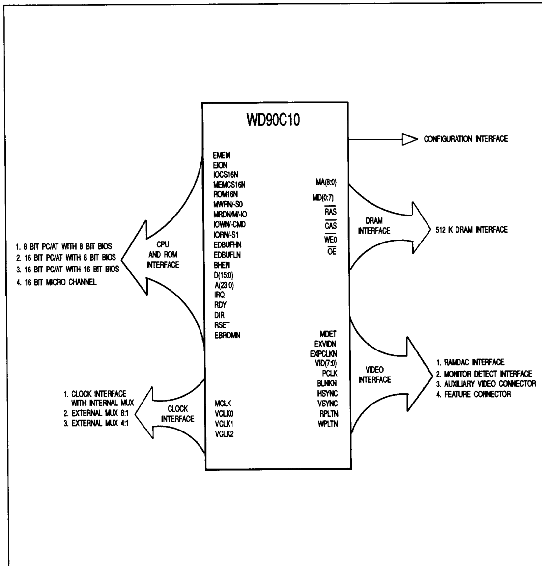
FIGURE 9. WD90C10 INTERFACES
