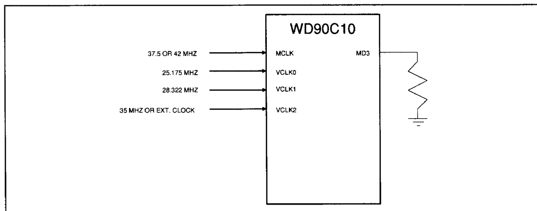
FIGURE 17. CLOCK INTERFACE
