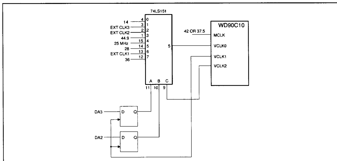
FIGURE 18. EXTERNAL VIDEO CLOCK MULTIPLEXING
